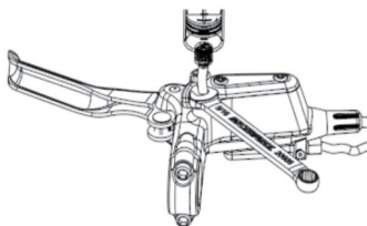
Figure 5-3: 8mm open end spanner to loosen/tighten the main body of the caliper into the nozzle screws.
