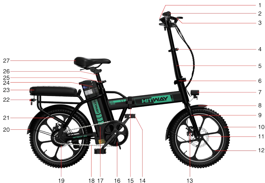
Figure 1 (Whole vehicle diagram)
