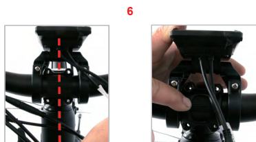
6. Place the handlebar into the tube and center the handlebar angle. Then close the front cover. NOTE: Do not twist the wire harness.
