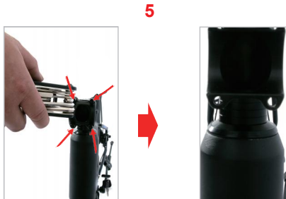
5. Remove the 4 front cover screws with the No. 4 Allen key in the 16-in-1 tool and remove the tube front cover.
